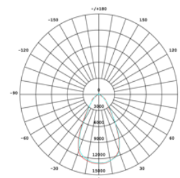
12x12 B/Angle BMP-5STAD60-800-15054-10D4
