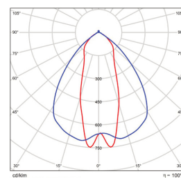
90x40 B/Angle BMP-RCAN2211-150-15057-10D
