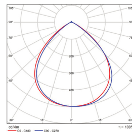
90x90 B/Angle BMP-3RCAN90-150-15057-10D
