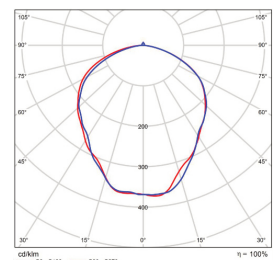
120x120 B/Angle BMP-3RCAN120-12015057-10
