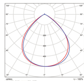
90x90 B/Angle BMP-3RCAN90-120-15057-10
