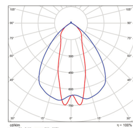
90x40 B/Angle BMP-3RCAN2211-120-15057-10
