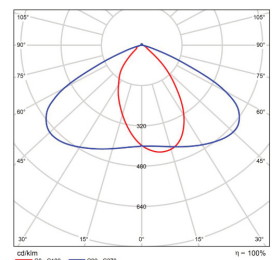
Tunnel Module BMP-3RCAN2123-100-15057-10
