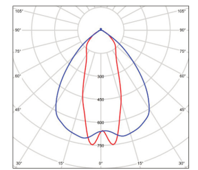
90x40 B/Angle BMP-FLMOD2211-120-15057-10
