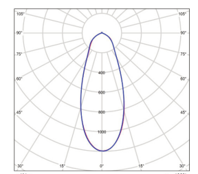
40x40 B/Angle BMP-FLMOD40-120-15057-10
