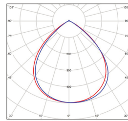
90x90 B/Angle BMP-FLMOD90-120-15057-10
