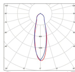
25x25 B/Angle BMP-FLMOD25-120-15057-10
