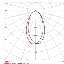
60x60 B/Angle BMP-HB60-150-150V-10
