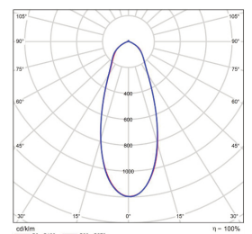
40x40 B/Angle BMP-HB40-150-150V-10
