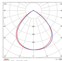
90x90 B/Angle BMP-HB90-150-150V-10
