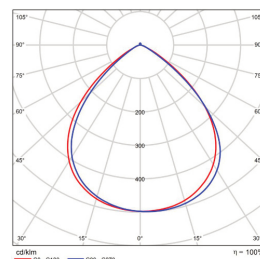
90x90 B/Angle BMP-HB90-40-150V-10
