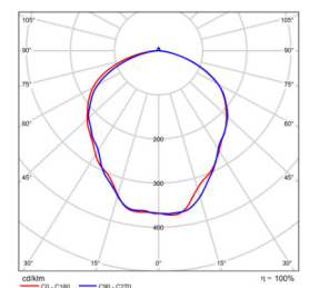
120x120 B/Angle BMP-HB120-40-150V-10
