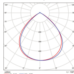
90x90 B/Angle BMP-HB90-50-150V-10
