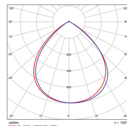
90x90 B/Angle BMP-HB90-60-150V-10
