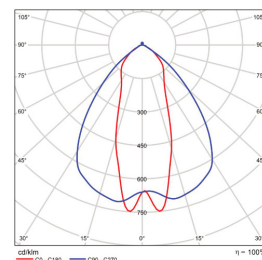
90x40 B/Angle BMP-HB2211-60-150V-10 Pallet racking isles
