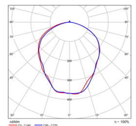
120x120 B/Angle BMP-HB120-60-150V-10
