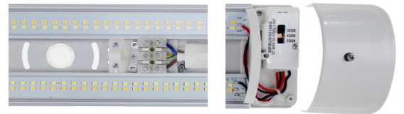
Terminal block centre of batten
