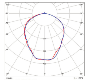
120x120 B/Angle BMP-SCAN120-100-15057-10
