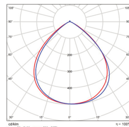
90x90 B/Angle BMP-SCAN90-100-15057-10
