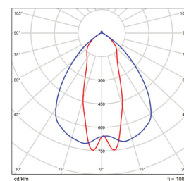
90x40 B/Angle BMP-SCAN2211-100-15057-10
