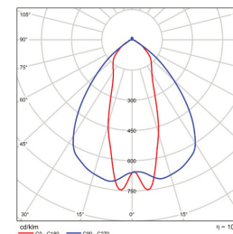
90x40 B/Angle BMP-SCAN2211-150-15057-10D
