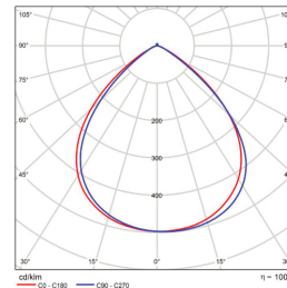
90x90 B/Angle BMP-SCAN90-150-15057-10D
