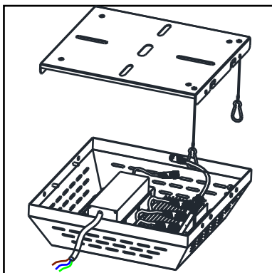
Mounting diagram
