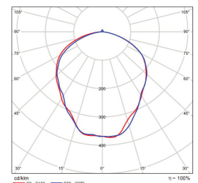
120x120 B/Angle BMP-SCAN120-180-15057-10D
