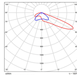
114x17 B/Angle BMP-STADL1251-400-150V-10
