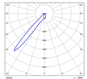
45x12 B/Angle BMP-STADL2318-400-150V-10
