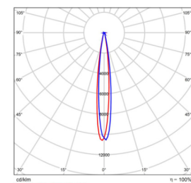
12x12 B/Angle BMP-STADL12-400-150V-10D4
