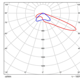
114x17 B/Angle BMP-STADL1251-400-150V-10D4
