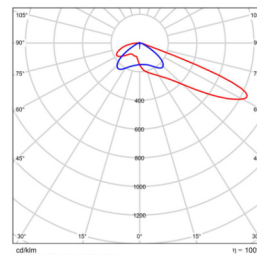
114x17 B/Angle BMP-STADL1251-500-150V-10D4 45x12 B/Angle BMP-STADL2318-500-150V-10D4
