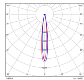
12x12 B/Angle BMP-STADL12-600-150V-10D4
