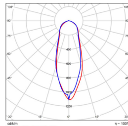
25 X 25 B/Angle BMP-STAD25-500-150V-10
