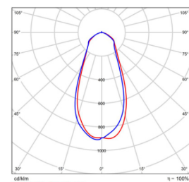
60x60 B/Angle BMP-STAD60-500-150V-10
