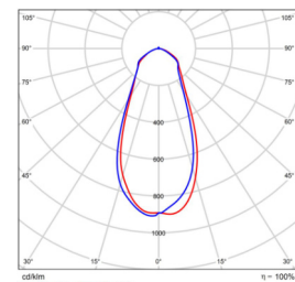
60x60 B/Angle BMP-STAD60-500-150V-10D4
