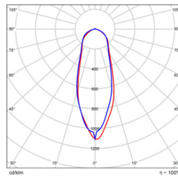
25 X 25 B/Angle BMP-STAD25-600-150V-10
