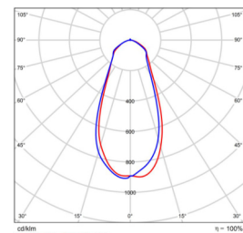
60x60 B/Angle BMP-STAD60-600-150V-10
