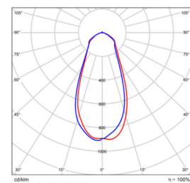
60x60 B/Angle BMP-STAD60-600-150V-10D4
