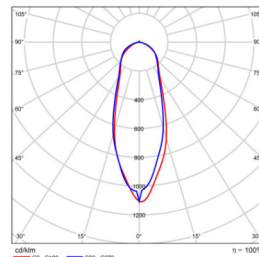
25 X 25 B/Angle BMP-STAD25-600-150V-10D4
