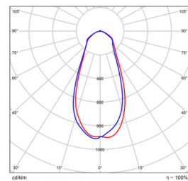
60x60 B/Angle BMP-STAD60-800-150V-10
