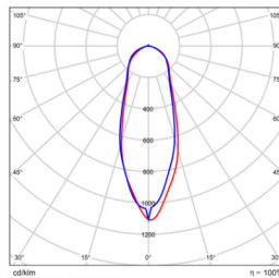
25 X 25 B/Angle BMP-STAD25-800-150V-10
