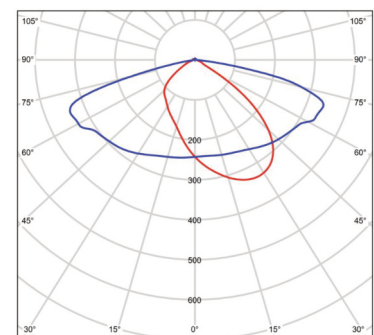
Type II (Most Common) BMP-STREET2-240-150V-10
