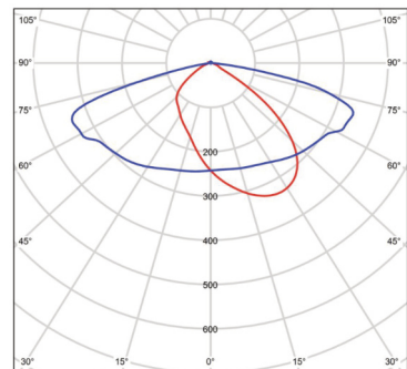
Type II (Most Common) BMP-STREET24VDC2-100-150V-10
