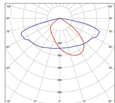
Type II (Most Common) BMP-STREET24VDC2-150-150V-10
