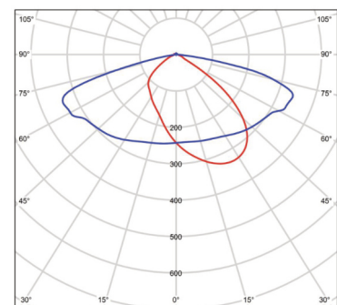
Type II (Most Common) BMP-STREET24VDC2-60-150V-10
