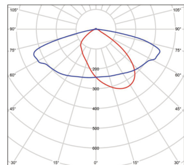
Type II (Most Common) BMP-STREET2-100-150V-10
