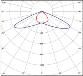
Type I BMP-STREET1-40-150V-10
