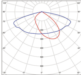
Type II BMP-STREET2-40-150V-10 (Most Common)
