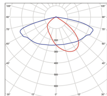
Type II (Most Common) BMP-STREET2-40-150V-10
