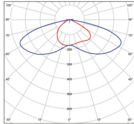
Type III BMP-STREET3-40-150V-10
