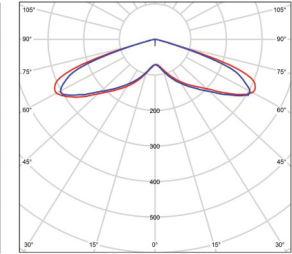
Type V BMP-STREET5-40-150V-10
