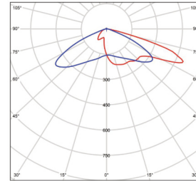
Type IV BMP-STREET4-40-150V-10
