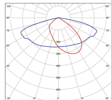
Type II (Most Common) BMP-STREET2-50-150V-10
