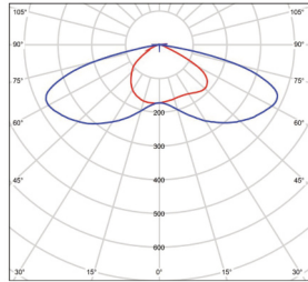
Type III BMP-STREET3-50-150V-10
