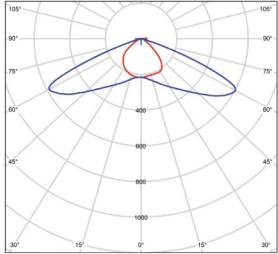
Type I BMP-STREET1-50-150V-10
