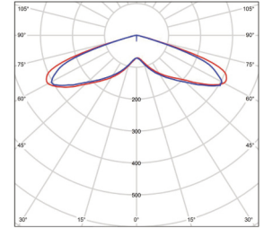
Type V BMP-STREET5-50-150V-10
