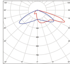
Type IV BMP-STREET4-50-150V-10
