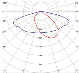
Type II BMP-STREET2-50-150V-10 (Most Common)
