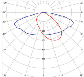
Type II BMP-STREET2-80-150V-10 (Most Common)
