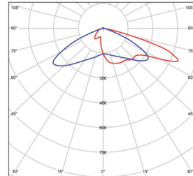
Type IV BMP-STREET4-80-150V-10
