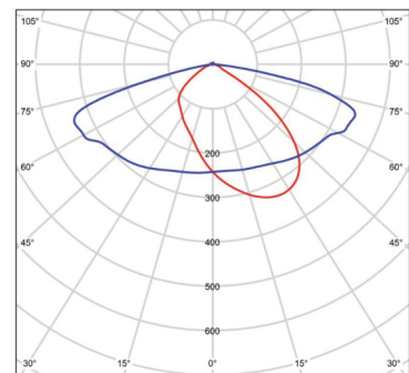
Type II (Most Common) BMP-STREET2-80-150V-10
