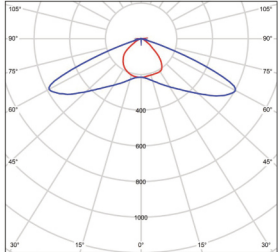
Type I BMP-STREET1-80-150V-10
