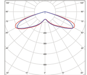
Type V BMP-STREET5-80-150V-10
