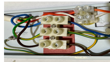
PA16H Large terminal Block
