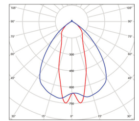
90x40 B/Angle BMP-FLMOD2211-40-15057-10
