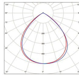
90x90 B/Angle BMP-FLMOD90-40-15057-10
